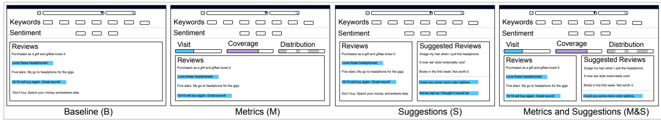
Figure 5: This figure depicts all Serendyze components and which features were available with the four conditions (B, M, S, and M&S). The dropdown for product selection, search options, keywords and sentiment filters, and reviews were available for all four conditions (B, M, S, and M&S). The exploration metrics (Visit, Coverage, and Distribution) were only available for conditions M and M&S. The suggestions generated by the bias mitigation model were only available for conditions S and M&S.
