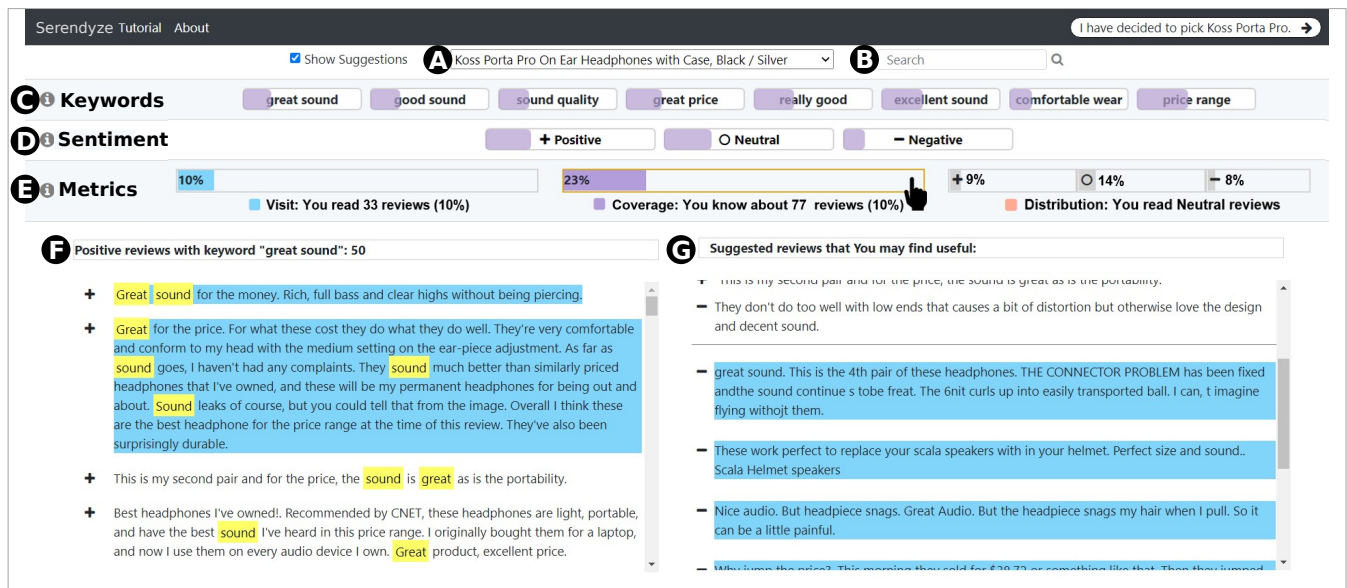
Figure 3: Different components in the Serendyze interface: A) a dropdown option for selecting a product, B) a search bar to search for any word present in the reviews, C) a set of filters corresponding to representative keywords, D) filters for positive, neutral, and negative reviews, E) the exploration metrics - Visit, Coverage, and Distribution, F) all product reviews and G) suggested reviews generated by the bias mitigation model that the readers may find interesting.
