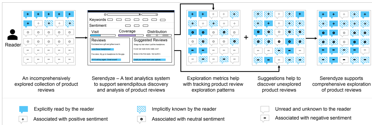
Figure 1: Serendyze is a text analytics system that uses two novel interventions – exploration metrics and a bias mitigation model – to enable readers to explore product reviews more comprehensively. The exploration metrics help readers track their data exploration across different facets, such as sentiments. The bias mitigation model suggests reviews that are semantically and sentiment-wise dissimilar to what the readers have been exploring so that they can discover a broader range of reviews. Integrated within an interactive interface, these features can enable readers to gain comprehensive knowledge about the data prior to decision-making.
