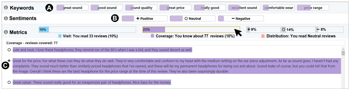
Figure 4: Hovering over the Visit or Coverage metric bars reveals data exploration scented widgets embedded in the keyword (A) and sentiment filters (B). Here, the reader hovered over the Coverage bar, and the scented widgets show the keyword pair “comfortable wear” and the negative reviews are underexplored compared to other keyword pairs and sentiments. Clicking on the bar filters shows reviews (C) relevant to the exploration metric selected.
