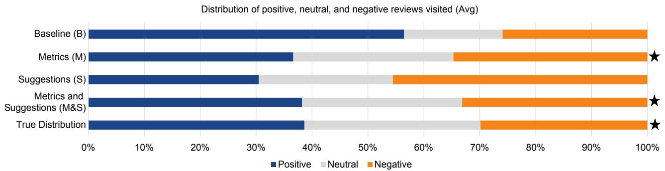
Figure 7: This figure depicts the average distribution of positive, negative, and neutral reviews as visited by participants. The figure suggests that participants in conditions M and M&S, annotated by (★), explored different sentiments in a balanced manner, which is reflective of the true distribution of sentiments present in the dataset. However, in the other two cases, we see an imbalance where participants in condition B visited a relatively larger number of positive reviews, and the participants in condition S visited a relatively larger number of negative reviews.
