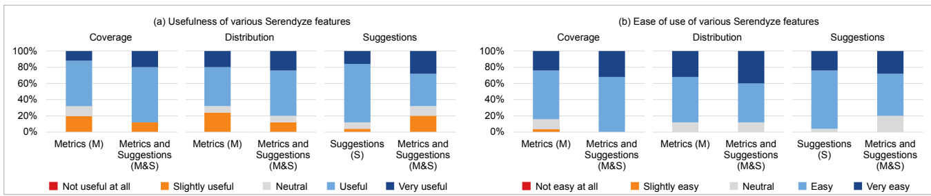
Figure 9: This figure depicts how the participants perceived the (a) usefulness and (b) ease of use of Coverage, Distribution, and suggestions based on the conditions where the participants had access to these features. The figure suggests that the usefulness of all features is over 68%, and ease of use is over 80% across all relevant conditions.
